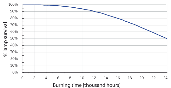
Lamp Survival CMH Streetwise™ 50W EM, 70W & 150W
