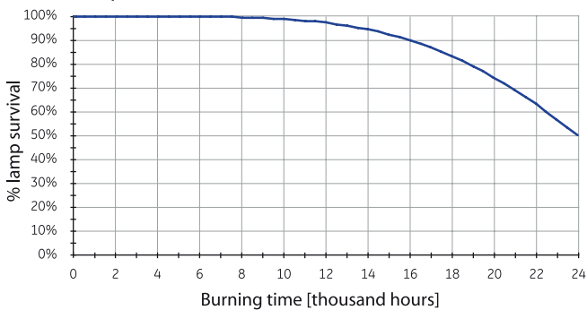
Lamp Survival CMH Streetwise™ 50W ECG & 100W
