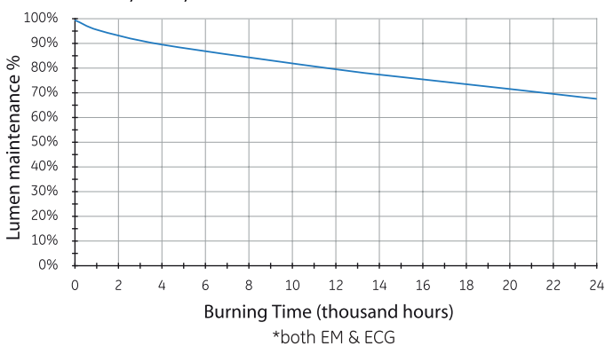
Lumen Maintenance CMH Streetwise™ 50W*, 70W, 100W & 150W
